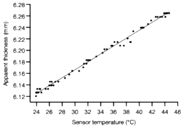
Figure 2. The relationship (Eq. 1) between the apparent thickness ( S_a ) of a temperature-insensitive Invar bar and the sensor temperature.
